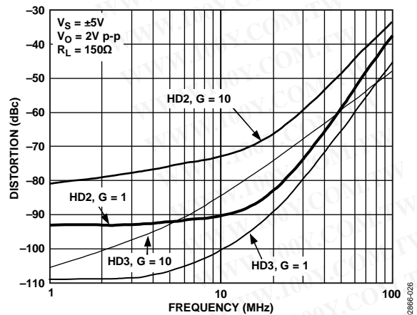
Figure 26. AD8008 Second and Third Harmonic Distortion vs. Frequency and Gain
