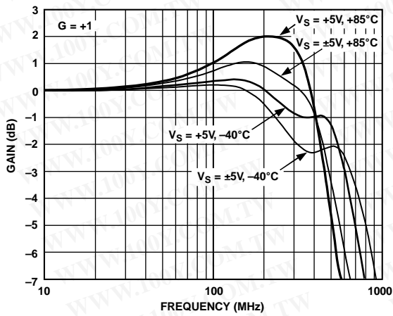
Figure 13. Small Signal Frequency Response over Temperature, V_S = +5V , V_S = \pm 5V
