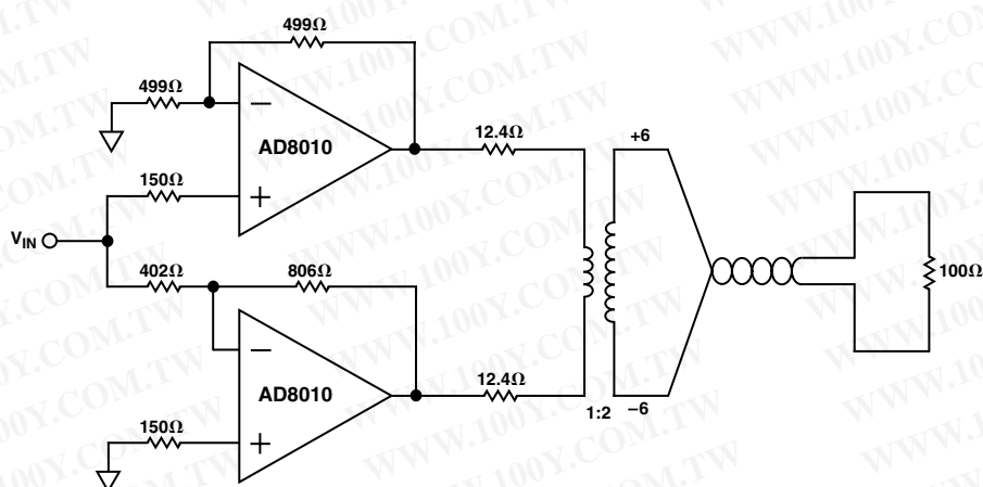
Figure 31. High Output Differential Line Driver Using Two AD8010s.
