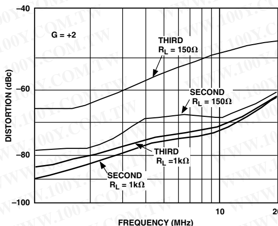
Figure 2. Distortion vs. Frequency; V S = \pm 5 V
