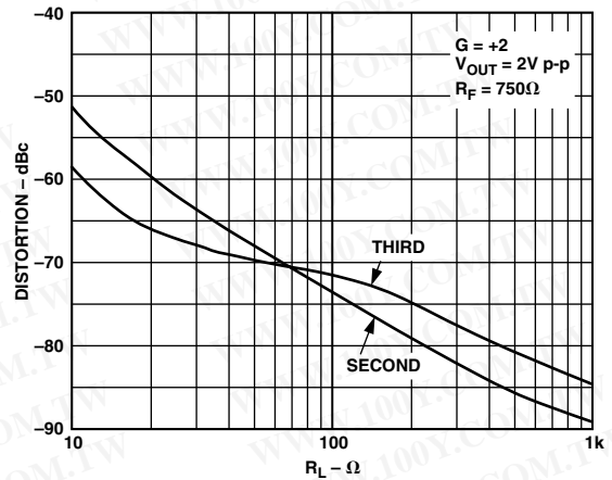
TPC 11. Distortion vs. Load Resistance; V_S = \pm 5\text{ V} , Frequency = 500 kHz
