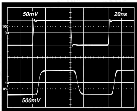
Figure 21. Large Signal Pulse Response, Gain = +10, R_F = 301 \Omega , R_L = 150 \Omega , V_S = \pm 5 \text{ V}
