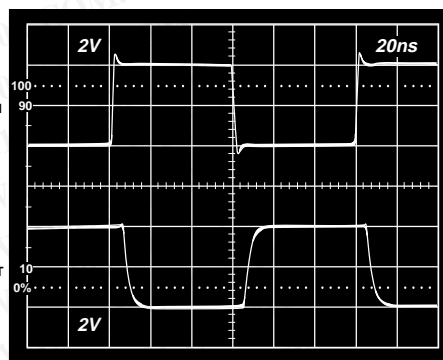
Figure 24. Large Signal Pulse Response, Gain = -1, (R_F = 698 \Omega, R_L = 150 \Omega, V_S = \pm 5 \text{ V})
