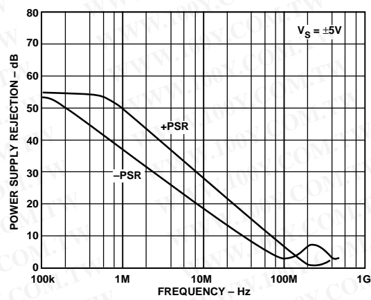
Figure 13. Power Supply Rejection Ratio vs. Frequency
