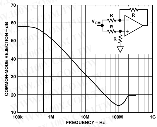
Figure 12. Common-Mode Rejection vs. Frequency
