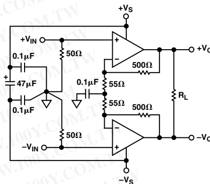
TPC 4. Differential Test Circuit; G = +10
