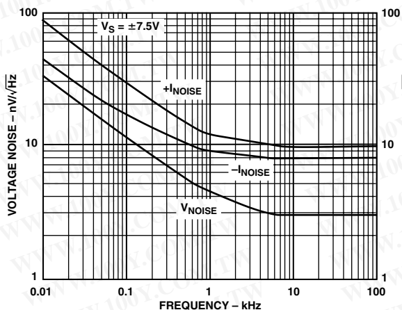
TPC 8. Input Current and Voltage Noise vs. Frequency
