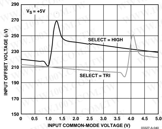
Figure 41. Input Offset Voltage vs. Input Common-Mode Voltage, V_S = 5
