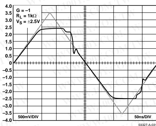
Figure 32. Output Overdrive Recovery
