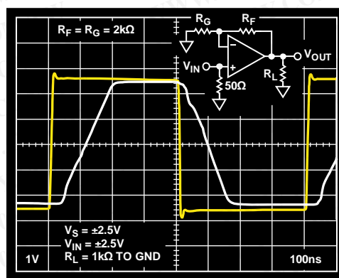
Figure 45. Overdrive Recovery
