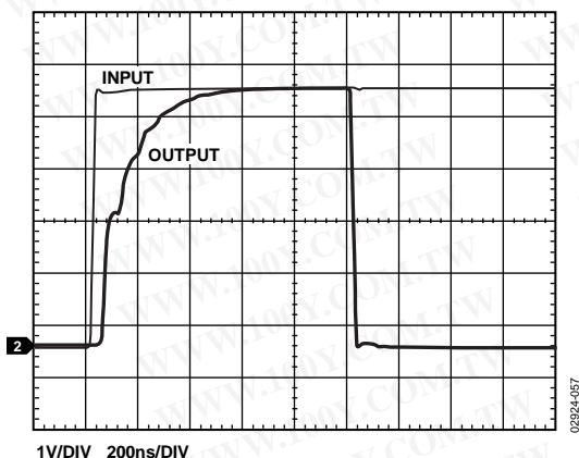
Figure 57. Peak Detector Response 5 V, 1 \mu s Pulse
