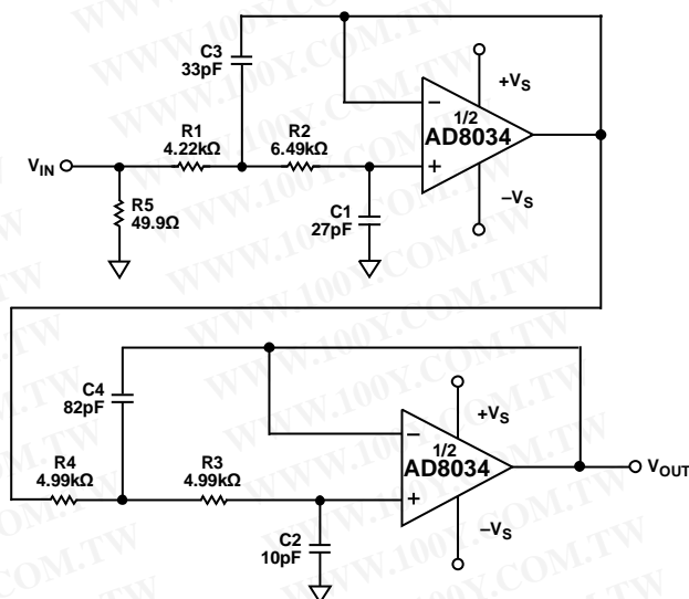
Figure 58. 4-Pole Cascade Sallen-Key Filter
