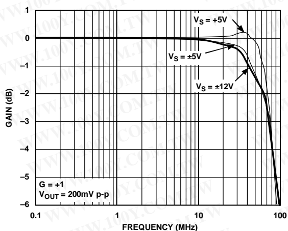
Figure 7. Small Signal Frequency Response for Various Supplies (See Figure 44)
