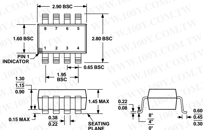
Figure 66. 8-Lead Small Outline Transistor Package [SOT-23]
