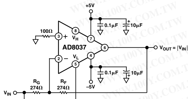
Figure 12. Full-Wave Rectifier
