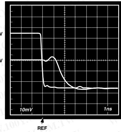
TPC 60. AD8037 Clamp Overdrive (2x) Recovery
