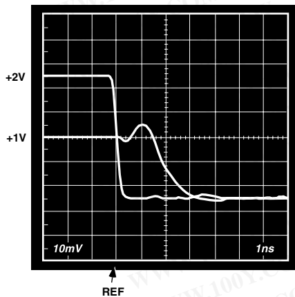
TPC 57. AD8036 Clamp Overdrive (2x) Recovery
