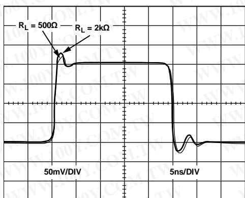
Figure 25. Small Signal Transient Response for Various R_L , V_S = 5\text{ V}
