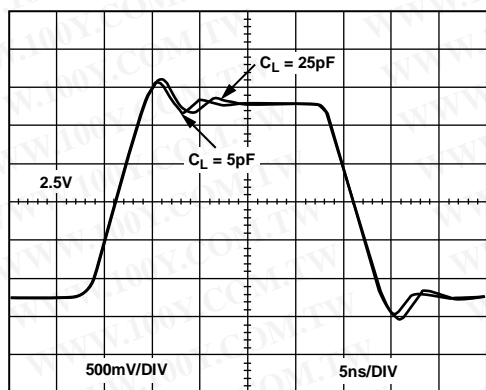
Figure 31. Large Signal Transient Response for Various C_L , V_S = \pm 5V
