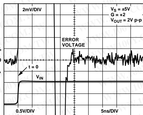
Figure 35. 0.1% Settling Time V_{OUT} = 2V p-p
