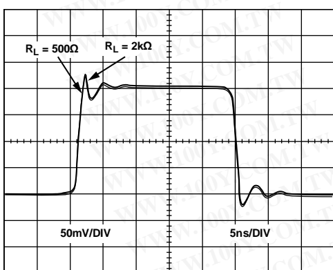
Figure 26. Small Signal Transient Response for Various R_L , V_S = \pm 5\text{ V}
