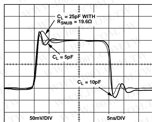
Figure 28. Small Signal Transient Response for Various C_L , V_S = \pm 5\text{ V}
