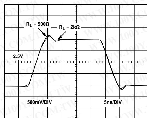
Figure 29. Large Signal Transient Response for Various R_L , V_S = 5\text{ V}
