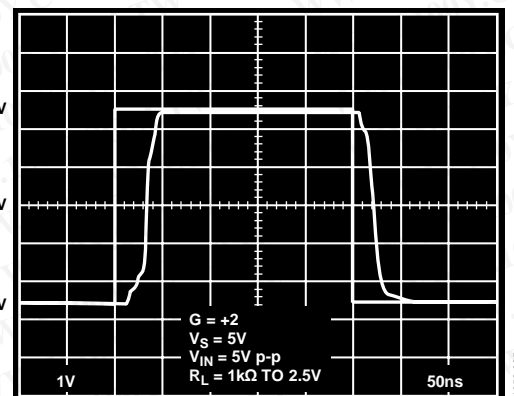
Figure 37. Overdrive Recovery
