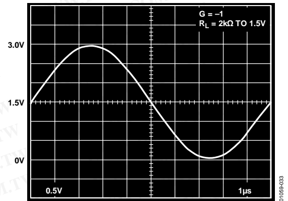
Figure 33. Rail-to-Rail Output Swing, V_S = 3\text{ V}
