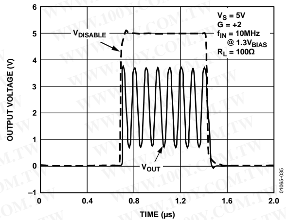
Figure 35. AD8063 \overline{DISABLE} Function, Voltage = 0 V to 5 V
