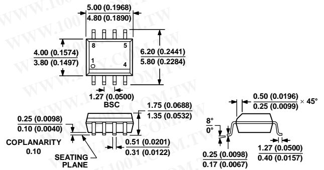
Figure 59. 8-Lead Standard Small Outline Package [SOIC_N] Narrow Body (R-8) Dimensions shown in millimeters and (inches)
