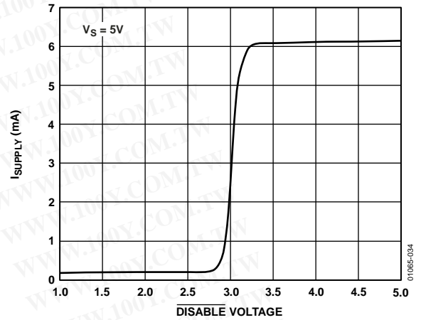
Figure 34. AD8063 \overline{DISABLE} Voltage vs. Supply Current
