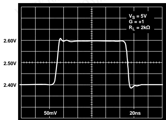
Figure 25. 200 mV Step Response; V_S = +5\text{ V} , G = +1
