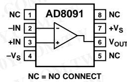
Figure 1. SOIC-8 (R-8)
