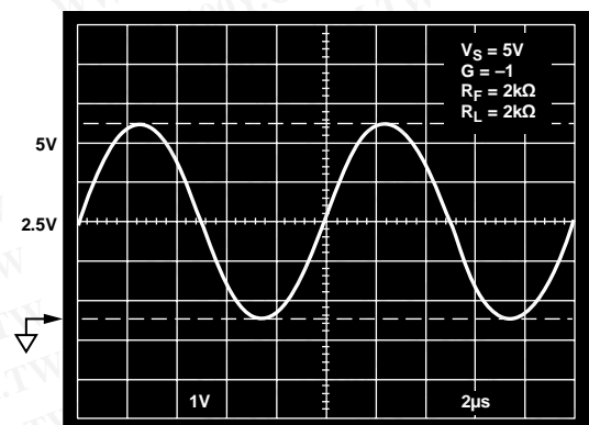
Figure 27. Output Swing; G = -1 , R_L = 2\text{ k}\Omega
