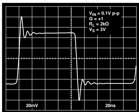
Figure 24. 100 mV Step Response; G = +1
