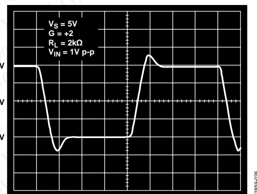
Figure 26. Large Signal Step Response; V_S = +5\text{ V} , G = +2
