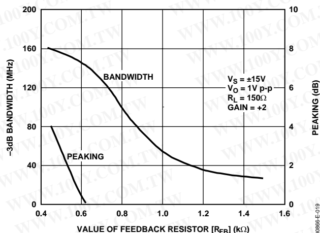
Figure 19. -3 dB Bandwidth and Peaking vs. Value of R_{FB}
