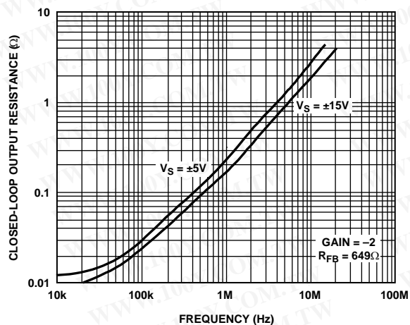
Figure 15. Closed-Loop Output Resistance vs. Frequency
