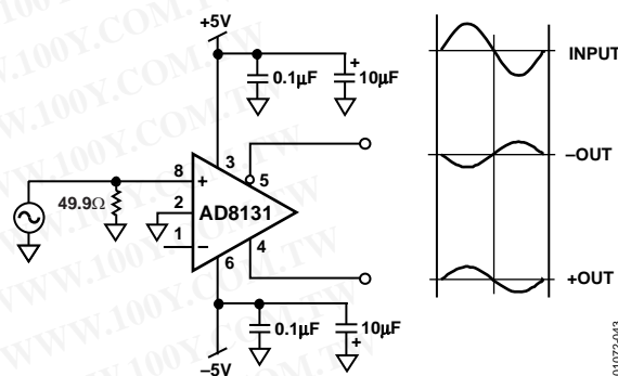
Figure 43. Unity Gain, Single-Ended-to-Differential Amplifier
