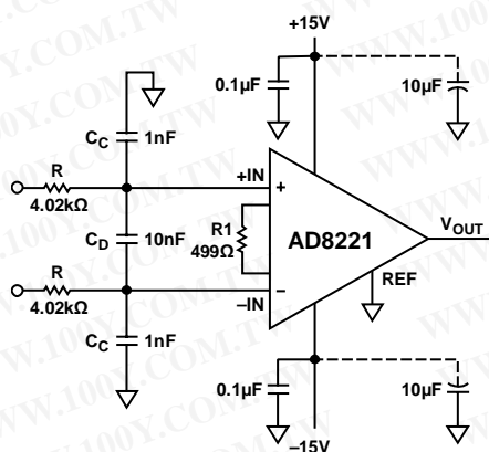
Figure 48. RFI Suppression
