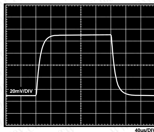
Figure 45. Small Signal Pulse Response, G = 1000 , R_{LOAD} = 2\text{ k}\Omega , C_{LOAD} = 100\text{ pF} , V_S = \pm 15\text{ V} , V_{REF} = 0\text{ V}
