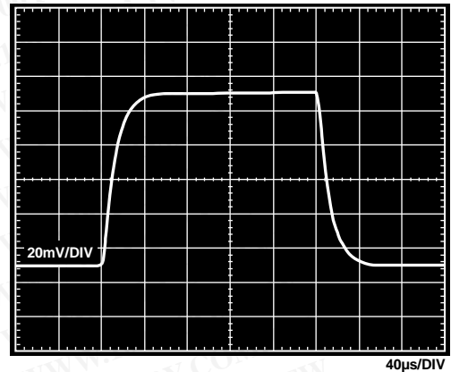
Figure 49. Small Signal Pulse Response, G = 1000 , R_{LOAD} = 2\text{ k}\Omega , C_{LOAD} = 100\text{ pF} , V_S = 5\text{ V} , V_{REF} = 2.5\text{ V}
