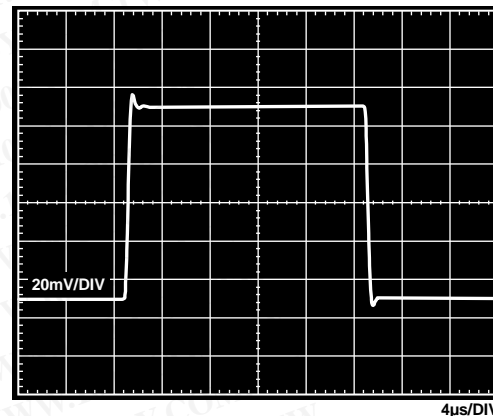
Figure 43. Small Signal Pulse Response, G = 10 , R_{LOAD} = 2\text{ k}\Omega , C_{LOAD} = 100\text{ pF} , V_S = \pm 15\text{ V} , V_{REF} = 0\text{ V}
