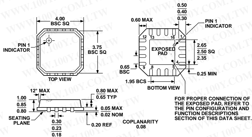
Figure 67. 16-Lead Lead Frame Chip Scale Package [LFCSP_VQ]
