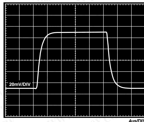
Figure 44. Small Signal Pulse Response, G = 100 , R_{LOAD} = 2\text{ k}\Omega , C_{LOAD} = 100\text{ pF} , V_S = \pm 15\text{ V} , V_{REF} = 0\text{ V}
