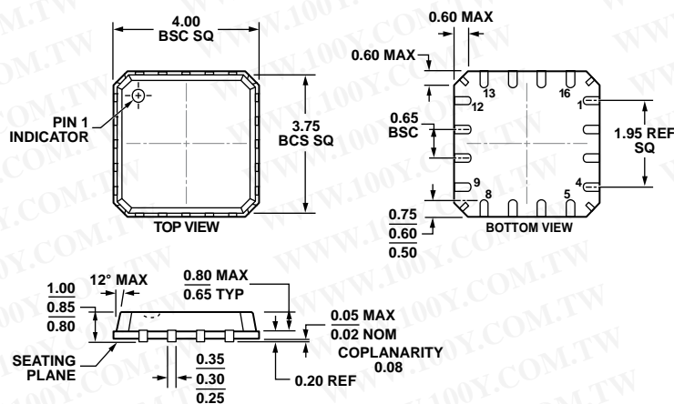
Figure 68. 16-Lead Lead Frame Chip Scale Package [LFCSP_VQ]
