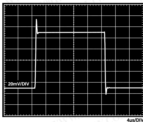
Figure 42. Small Signal Pulse Response, G = 1 , R_{LOAD} = 2\text{ k}\Omega , C_{LOAD} = 100\text{ pF} , V_S = \pm 15\text{ V} , V_{REF} = 0\text{ V}
