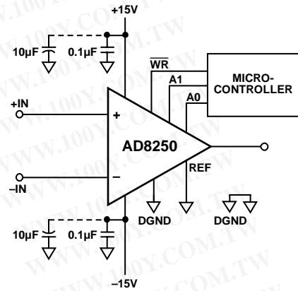
Figure 56. Programming Gain Using a Microcontroller
