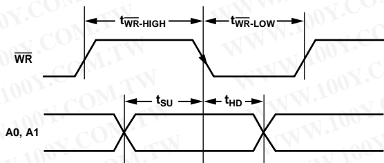
Figure 50. Timing Diagram for Latched Gain Mode
