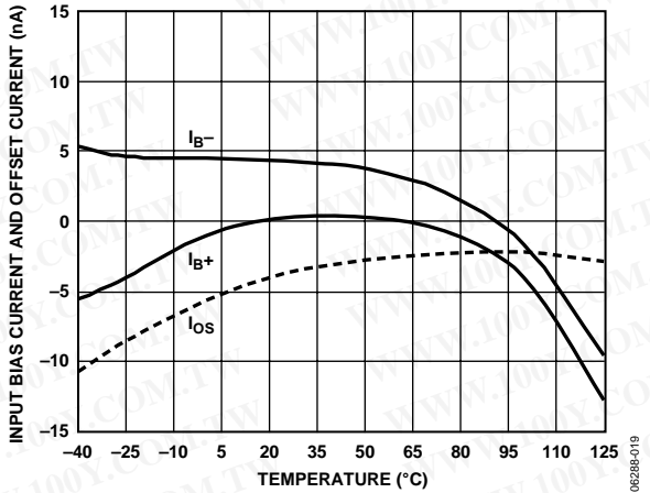
Figure 18. Input Bias Current and Offset Current vs. Temperature
