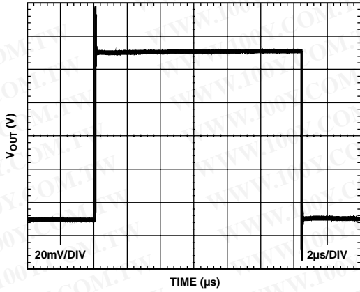
Figure 42. Small Signal Response G = 2, R_L = 2 \text{ k}\Omega, C_L = 100 \text{ pF}
