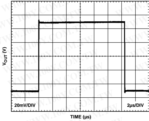
Figure 43. Small Signal Response G = 5, R_L = 2 \text{ k}\Omega, C_L = 100 \text{ pF}
