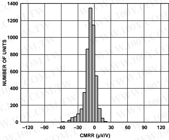
Figure 6. Typical Distribution of CMRR, G = 1
