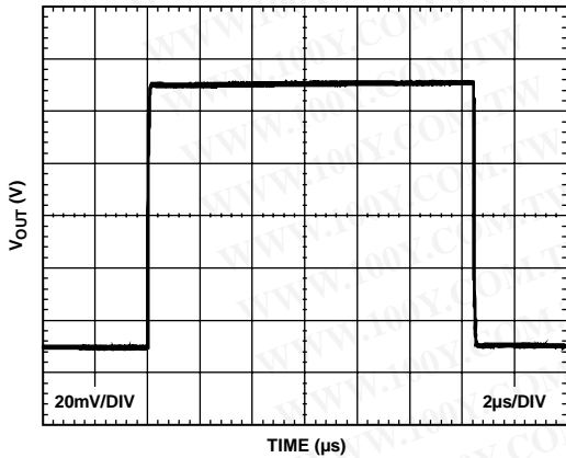
Figure 44. Small Signal Response, G = 10, R_L = 2 \text{ k}\Omega, C_L = 100 \text{ pF}
