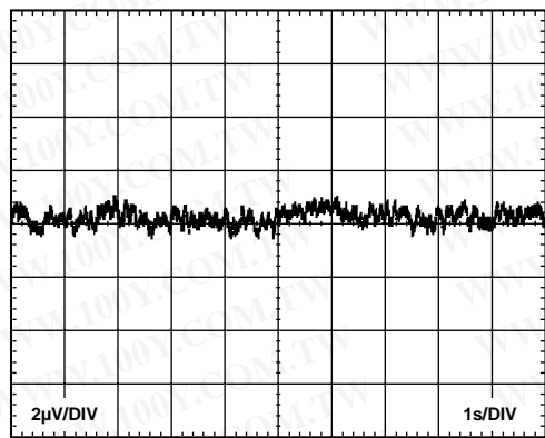
Figure 11. 0.1 Hz to 10 Hz RTI Voltage Noise, G = 1
