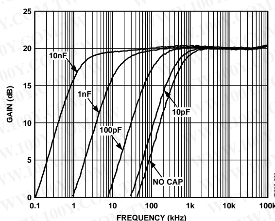
Figure 20. Gain vs. Frequency for Multiple Values of HPFL Capacitor at V_{GAIN} = 500\text{ mV}
