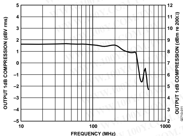
Figure 11. Output P1dB vs. Frequency at V_{GAIN} = 500 mV
