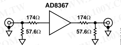
Figure 45. Characterization Test Setup
