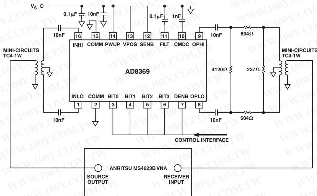
Figure 14. Vector Network Analyzer Setup (1 kΩ)
