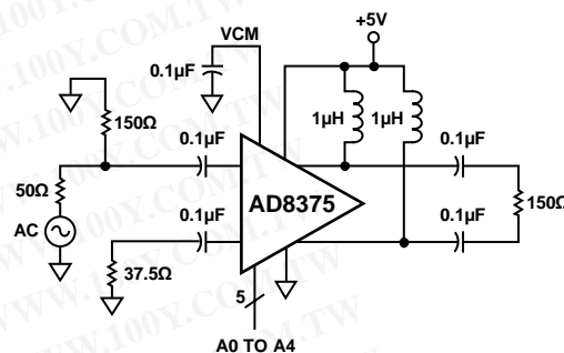
Figure 33. Single-Ended-to-Differential Conversion
