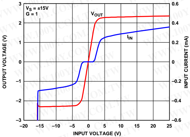
Figure 10. Input Overvoltage Performance, G = 1, V S = ±15 V
