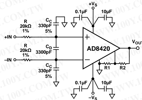
Figure 66. Suggested RFI Suppression Filter
