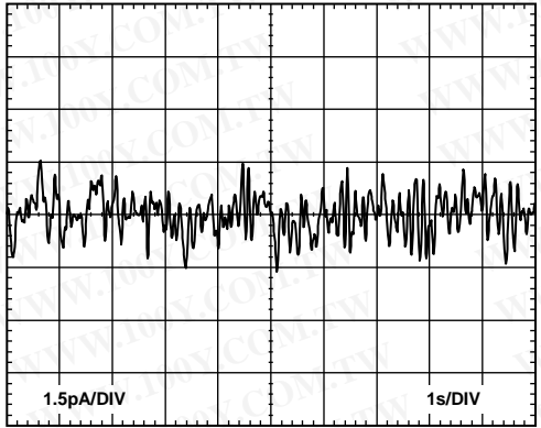
Figure 46. 0.1 Hz to 10 Hz Current Noise
