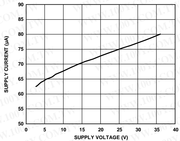
Figure 56. Supply Current vs. Supply Voltage
