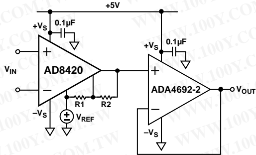
Figure 67. Output Buffering
