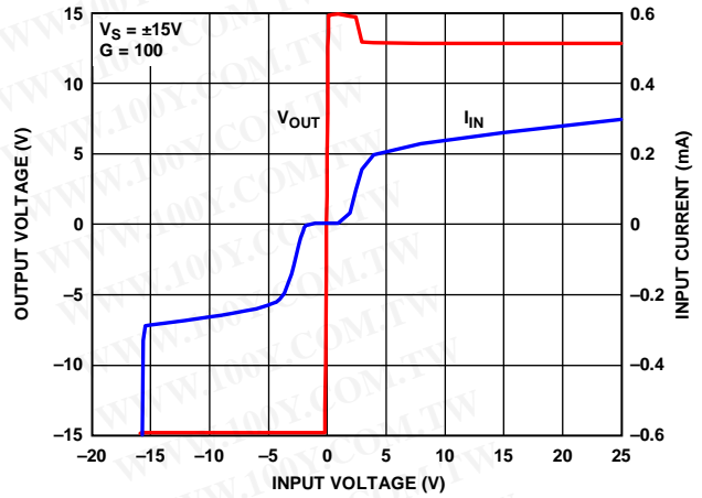
Figure 12. Input Overvoltage Performance, G = 100, V S = ±15 V
