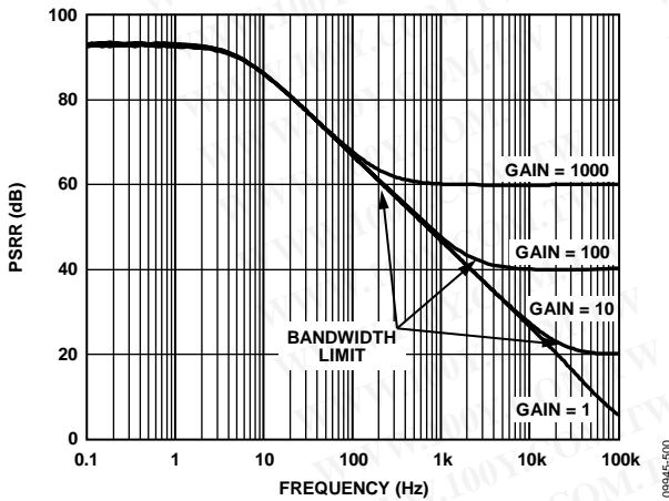
Figure 23. PSRR vs. Frequency on 5 V Supply
