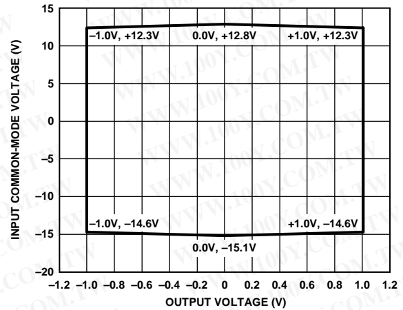
Figure 13. Input Common-Mode Voltage vs. Output Voltage, G = 1, V S = ±15 V
