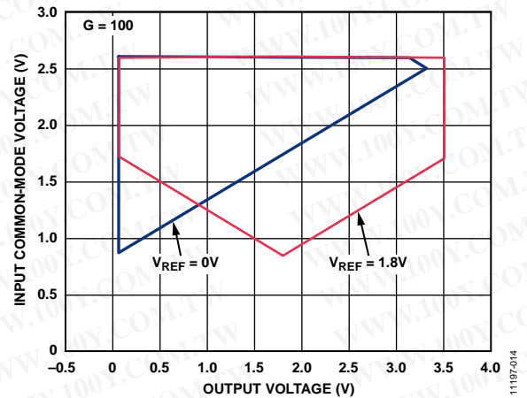
Figure 15. Input Common-Mode Voltage vs. Output Voltage ( G = 100 ), Single-Supply, V_S = 3.6\text{ V}
