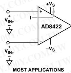
Figure 62. Input Overvoltage Protection with no External Components
