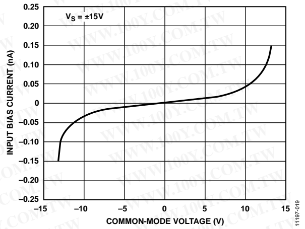
Figure 20. Input Bias Current vs. Common-Mode Voltage, V_S = \pm 15V
