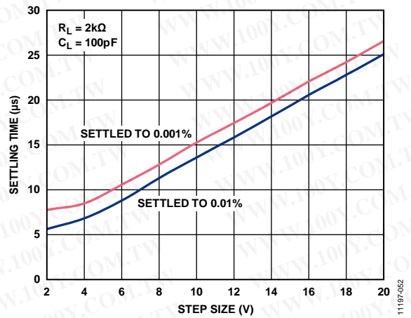
Figure 51. Settling Time vs. Step Size ( G = 1 )
