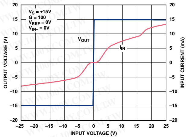
Figure 19. Input Overvoltage Performance; G = 100 , V_S = \pm 15V
