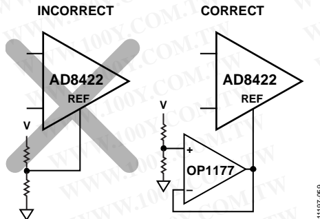
Figure 58. Driving the Reference Pin (REF)
