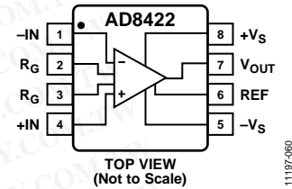
Figure 59. Pinout Diagram
