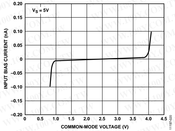
Figure 21. Input Bias Current vs. Common-Mode Voltage, V_S = 5V
