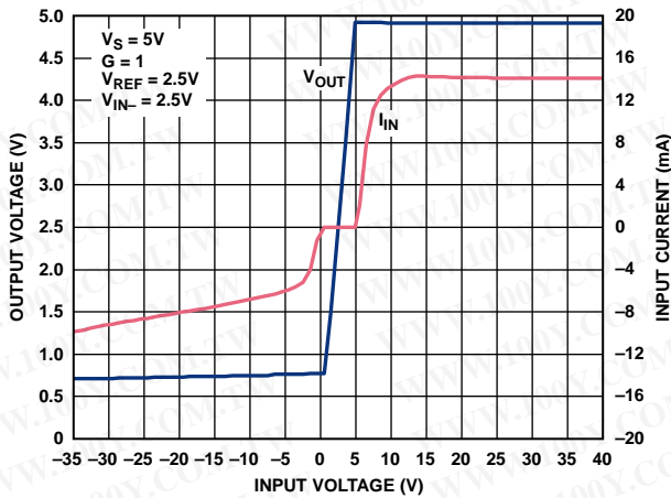
Figure 16. Input Overvoltage Performance; G = 1 , V_S = 5V
