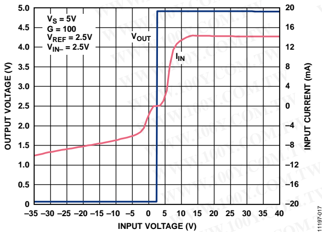
Figure 18. Input Overvoltage Performance; G = 100 , V_S = 5V
