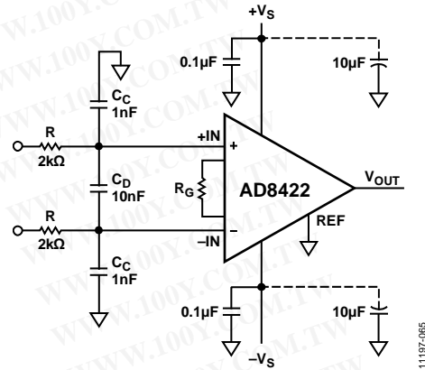
Figure 64. RFI Suppression
