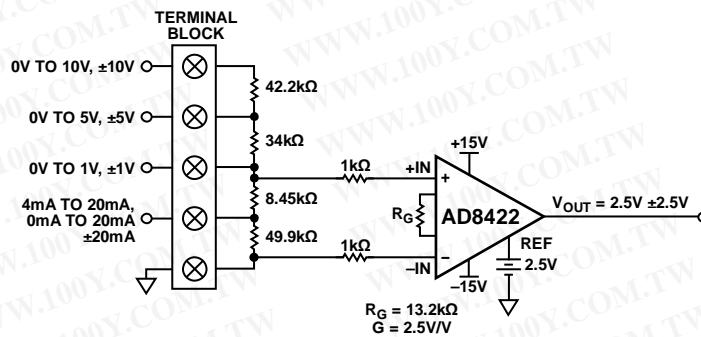
Figure 66. Process Control Analog Input
