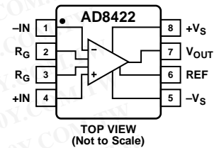
Figure 1. 8-Lead MSOP (RM), 8-Lead SOIC (R)
