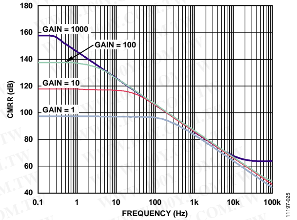
Figure 26. CMRR vs. Frequency, 1 kΩ Source Imbalance
