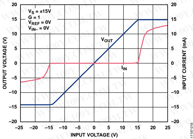
Figure 17. Input Overvoltage Performance; G = 1 , V_S = \pm 15V
