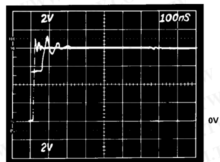
Figure 30. Peak Detector Response to 125 Hz Pulse Train
