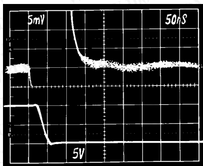
Figure 28. Settling Characteristics: +10 V to 0 V Step.
