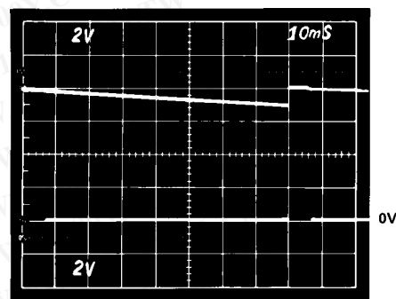
Figure 30. Peak Detector Response to 125 Hz Pulse Train
