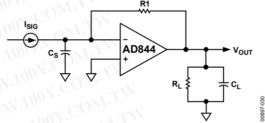
Figure 30. Current-to-Voltage Converter
