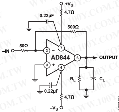
Figure 18. Gain of -10 Amplifier
