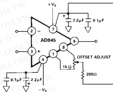
TPC 21. Offset Null Configuration
