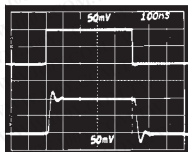
TPC 24. Unity Gain Follower Small Signal Pulse Response
