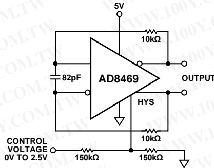
Figure 16. Voltage Controlled Oscillator
