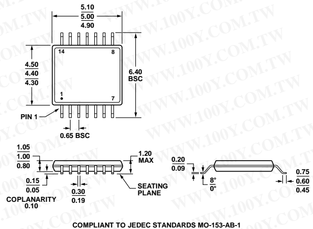
Figure 74. 14-Lead Thin Shrink Small Outline Package [TSSOP] (RU-14) Dimensions shown in millimeters
