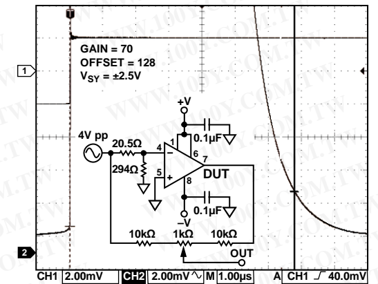
Figure 44. Settling Time 0.1%
