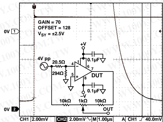
Figure 45. Settling Time 0.01%
