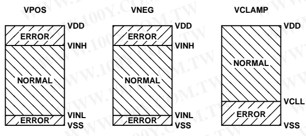
Figure 46. Voltage Regions at VPOS, VNEG, and VCLAMP that Trigger a Fault Condition
