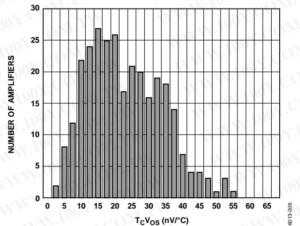
Figure 9. T_C V_{OS} at V_{SY} = 5V , -40^{\circ}C \leq T_A \leq +125^{\circ}C
