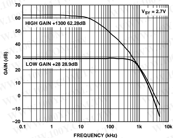
Figure 27. Closed-Loop Gain vs. Frequency Measured at Output Pin, V_{SY} = 2.7\text{ V}
