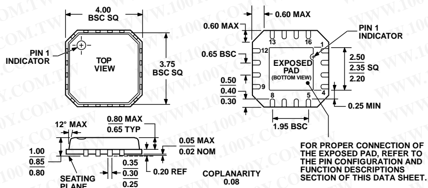
Figure 49. 16-Lead Lead Frame Chip Scale Package [LFCSP_VQ]
