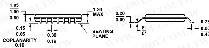
Figure 36. 14-Lead Thin Shrink Small Outline Package [TSSOP] (RU-14) Dimensions shown in millimeters
