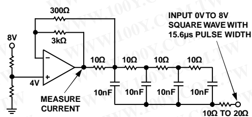
Figure 32. V_{\text{COM}} Test Circuit with Supply Voltage at 16 V
