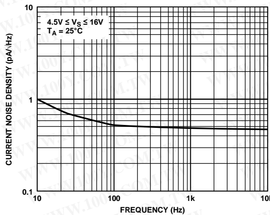
Figure 6. Current Noise
