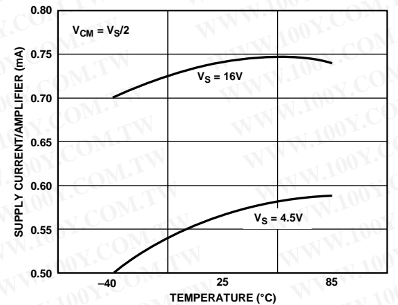
Figure 10. Supply Current/Amplifier vs. Temperature
