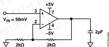
Figure 46. Capacitive Load Drive Test Circuit
