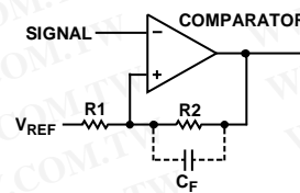
Figure 24. Configuring the AD8611/AD8612 with Hysteresis
