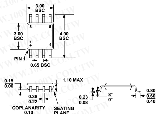
Figure 62. 8-Lead Mini Small Outline Package [MSOP] (RM-8)
