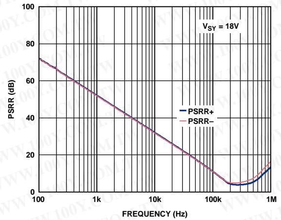
Figure 38. PSRR vs. Frequency
