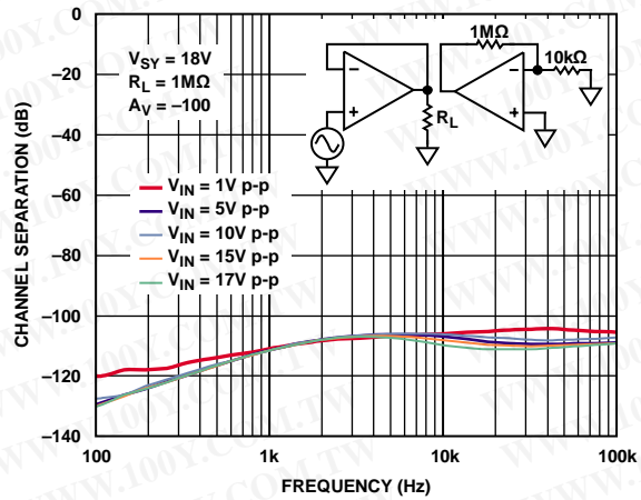
Figure 62. Channel Separation vs. Frequency
