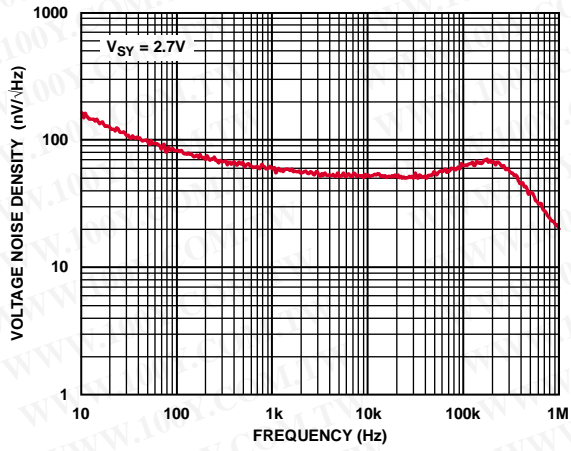
Figure 52. Voltage Noise Density vs. Frequency
