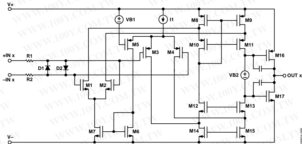
Figure 63. Simplified Schematic
