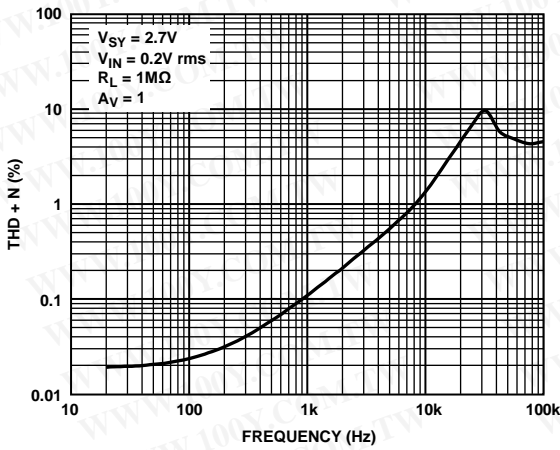
Figure 58. THD + N vs. Frequency
