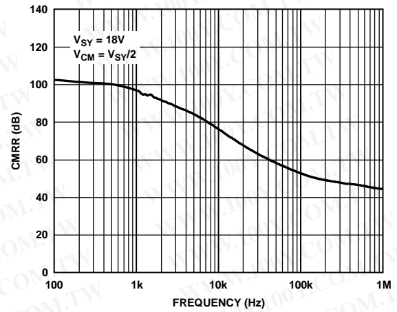
Figure 37. CMRR vs. Frequency
