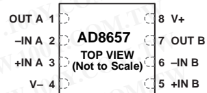
Figure 2. 8-Lead LFCSP
