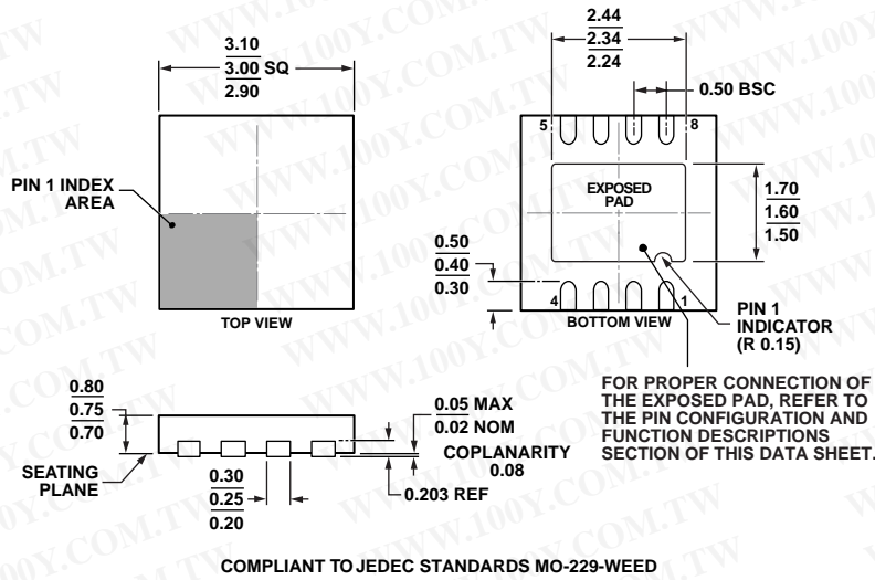
COMPLIANT TO JEDEC STANDARDS MO-229-WEED Figure 75. 8-Lead Lead Frame Chip Scale Package [LFCSP_WD] 3 mm x 3 mm Body, Very Very Thin, Dual Lead (CP-8-11) Dimensions shown in millimeters
