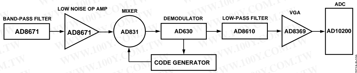
Figure 39. Simplified Block Diagram of a GPS Receiver
