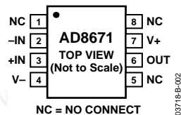
Figure 2. 8-Lead MSOP (RM-8)
