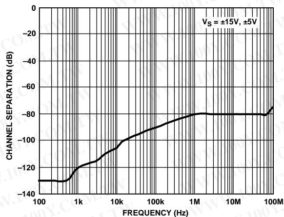
Figure 31. Channel Separation
