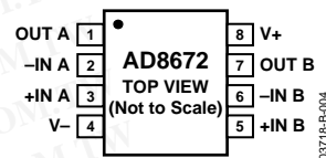
Figure 4. 8-Lead MSOP (RM-8)
