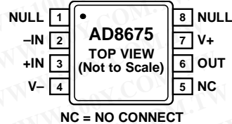
Figure 2. 8-Lead MSOP (RM-8)
