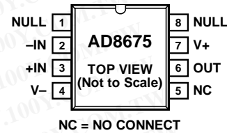
Figure 1. 8-Lead SOIC_N (R-8)
