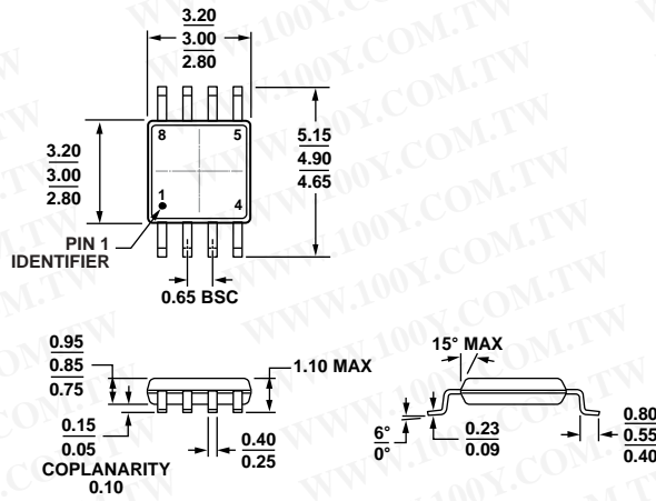
COMPLIANT TO JEDEC STANDARDS MO-187-AA Figure 30. 8-Lead Mini Small Outline Package [MSOP] (RM-8) Dimensions shown in millimeters
