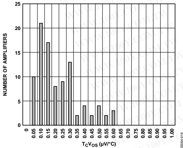
Figure 5. T_c V_{os}
