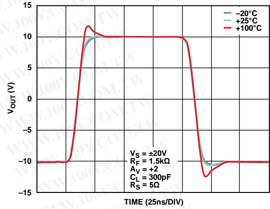
Figure 31. Large Signal Pulse Response vs. Case Temperature, A_v = +2 , V_s = \pm 20\text{ V} , V_{OUT} = 20\text{ V p-p} , R_f = 1.5\text{ k}\Omega , C_L = 300\text{ pF} , R_s = 5\ \Omega
