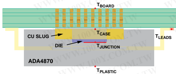
Figure 76. Thermal Model Stack-Up for Data in Table 7 (Heat Sink Not Shown)
