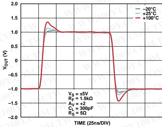
Figure 28. Small Signal Pulse Response vs. Case Temperature, A_v = +2 , V_s = \pm 5\text{ V} , V_{OUT} = 2\text{ V p-p} , R_f = 1.5\text{ k}\Omega , C_L = 300\text{ pF} , R_s = 5\ \Omega
