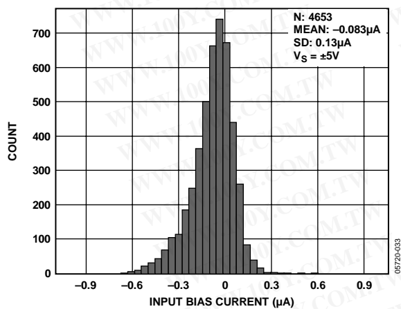
Figure 37. Input Bias Current Distribution
