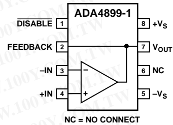
Figure 1. 8-Lead LFCSP_VD (CP-8-2)
