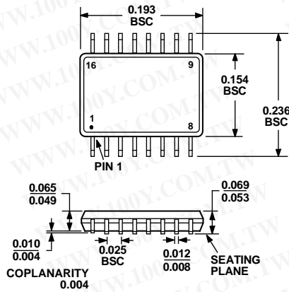
Figure 28. 16-Lead Shrink Small Outline Package [QSOP] (RQ-16) Dimensions shown in inches
