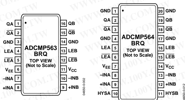
Figure 2. ADCMP563 16-Lead QSOP
