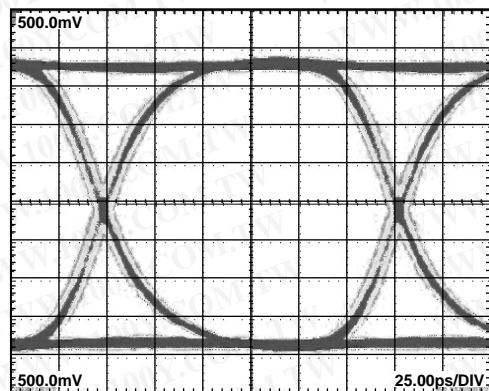
Figure 14. ADCMP572 Eye Diagram at 6.5 Gbps
