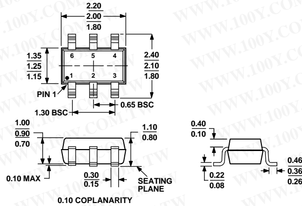
Figure 14. 6-Lead Thin Shrink Small Outline Transistor Package (SC70) (KS-6)
