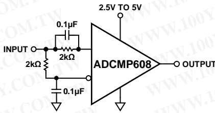
Figure 12. Self-Biased, 50% Slicer
