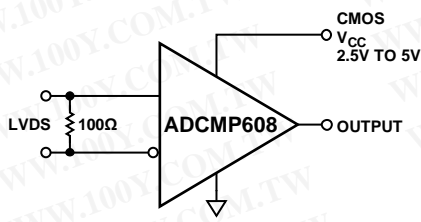
Figure 13. LVDS-to-CMOS Receiver
