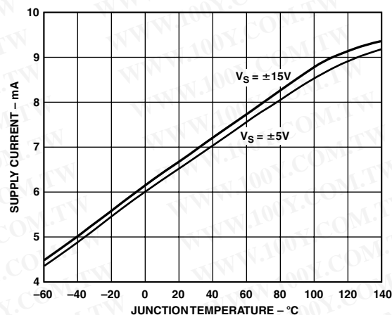
TPC 17. Supply Current vs. Junction Temperature
