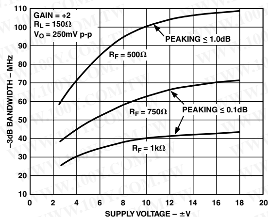
TPC 8. -3 dB Bandwidth vs. Supply Voltage, \text{Gain} = +2 , R_L = 150\ \Omega
