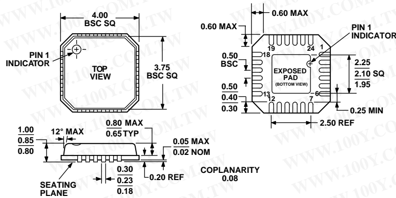
Figure 43. 24-Lead Lead Frame Chip Scale Package [LFCSFP] 4 mm × 4 mm Body (CP-24-1) Dimensions shown in millimeters
