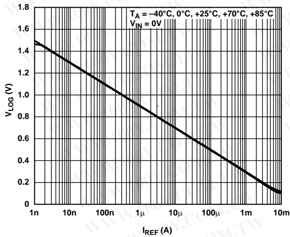
Figure 4. V_{LOG} vs. I_{REF} for Multiple Temperatures ( I_{INP} = 3\ \mu\text{A} )
