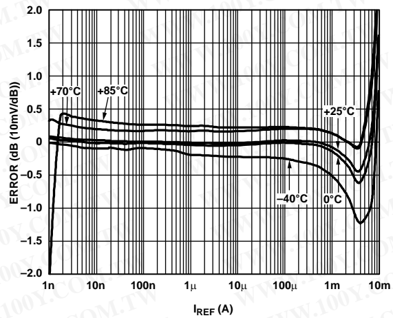
Figure 7. Law Conformance Error vs. I_{REF} for Multiple Temperatures, Normalized to 25^\circ\text{C} ( I_{INP} = 3\ \mu\text{A} )
