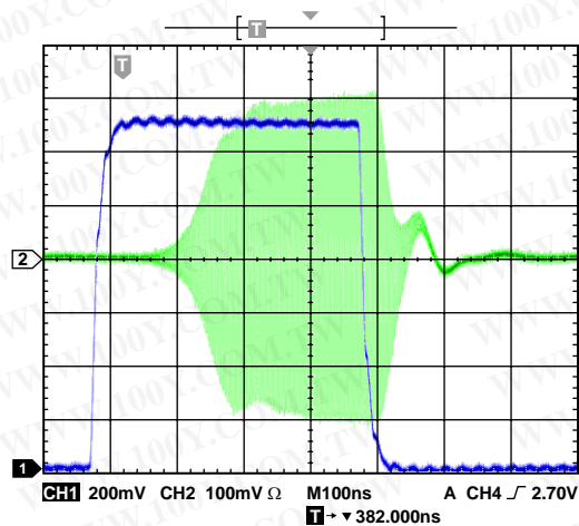
Figure 14. Step Response of Gain Control Input
