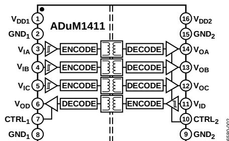
图2. ADuM1411
