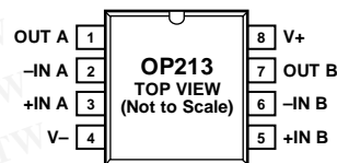
Figure 2. 8-Lead Narrow-Body SOIC_N
