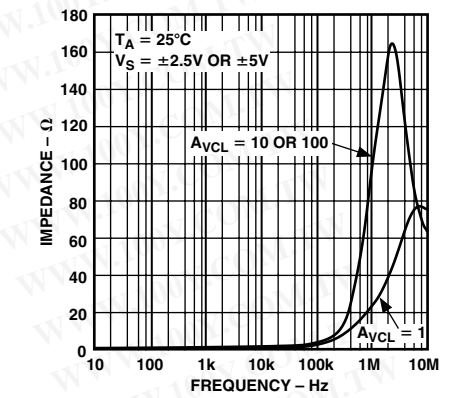
TPC 15. Closed-Loop Output Impedance vs. Frequency
