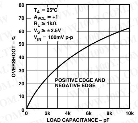
TPC 18. Small Signal Overshoot vs. Load Capacitance
